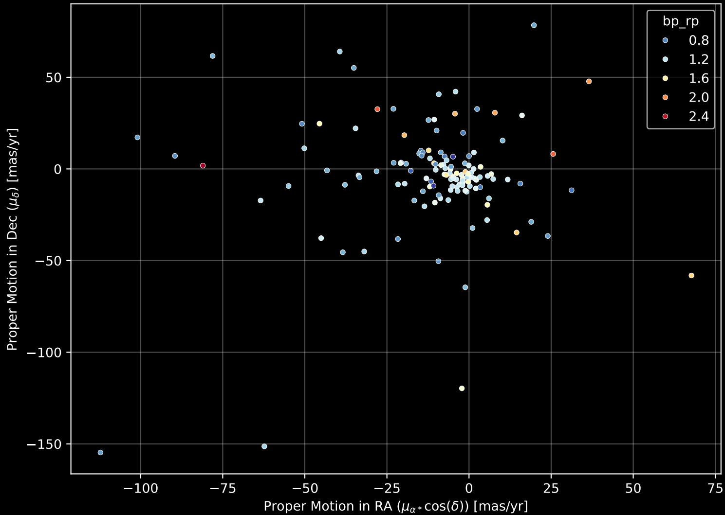
APOGEE DR17 Field: [042+45_MGA] Proper Motion Diagram (n= 135)
