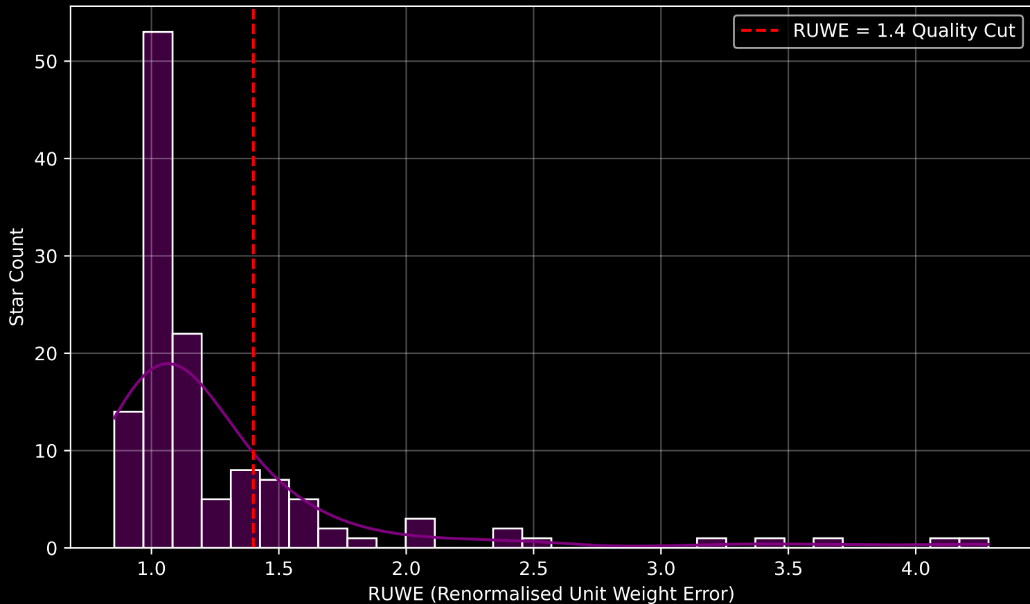
GAPOGEE DR17 Field [042+45_MGA] RUWE Distribution (n= 128)
