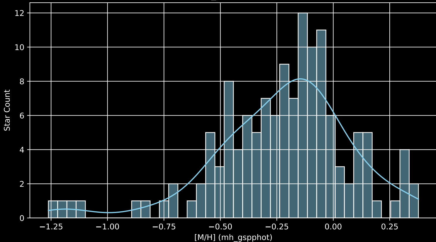
APOGEE DR17 Field: [042+45_MGA [M/H] (mh_gspphot) (n= 134)
