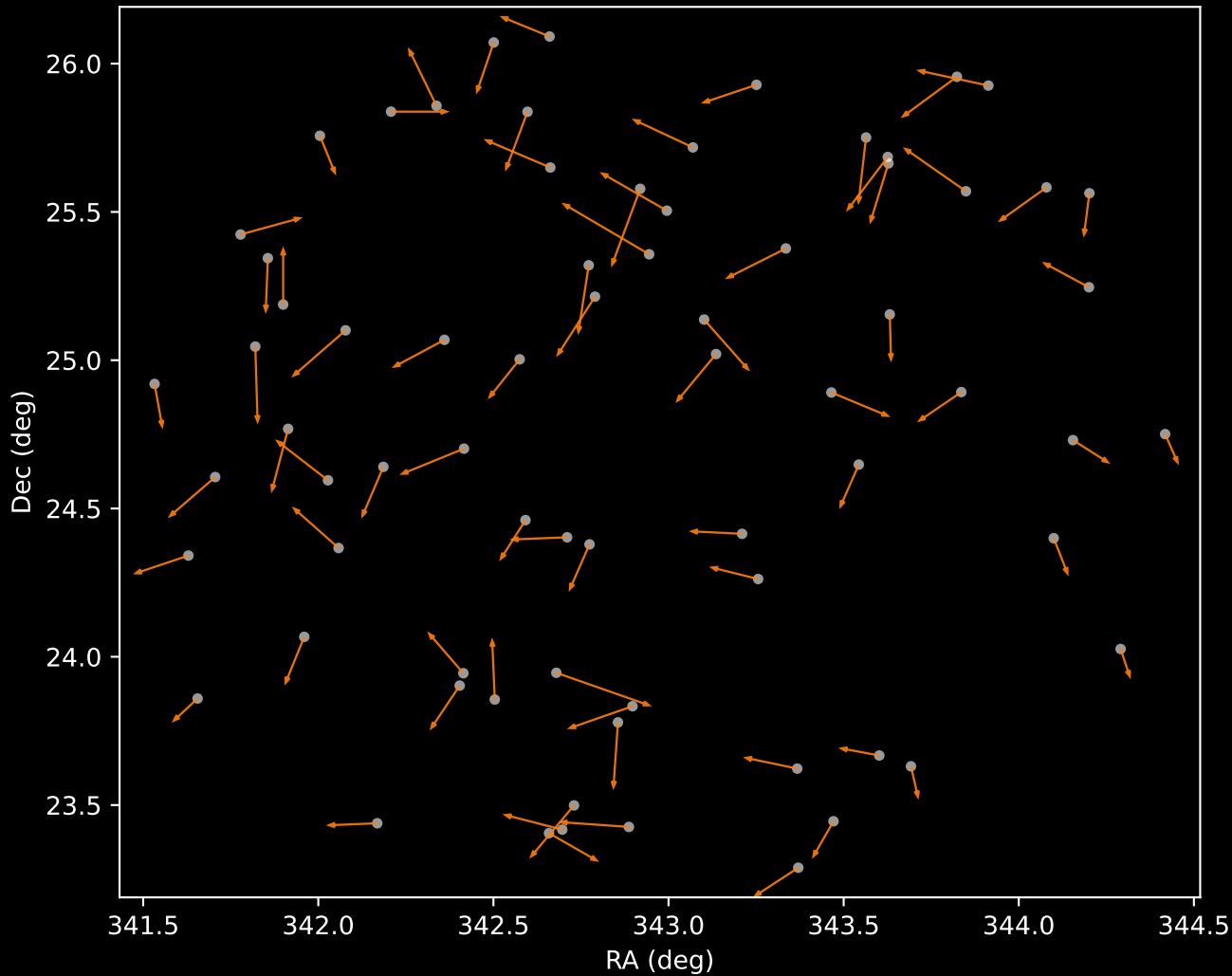
APOGEE DR17 Cluster 2 Proper Motion Vectors (n=72)
