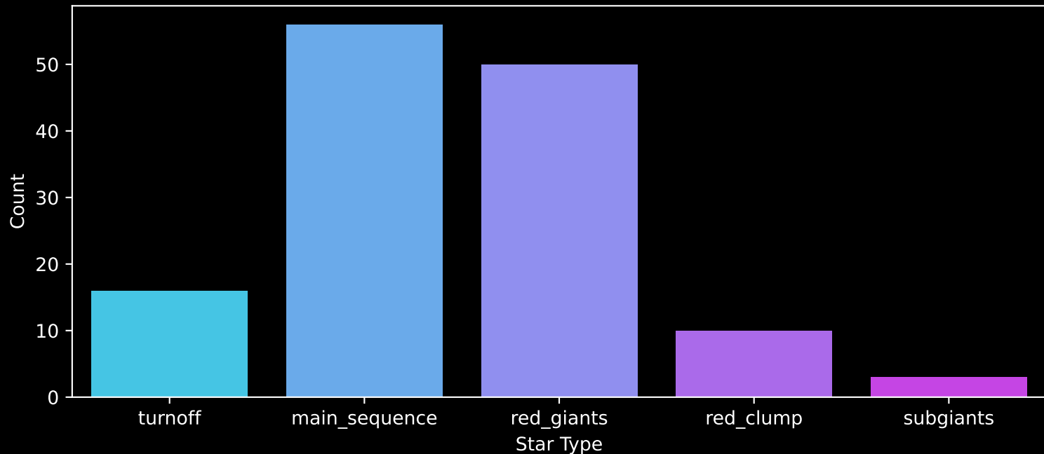
APOGEE DR17 Field: [042+45_MGA] Count plot of Star Type
