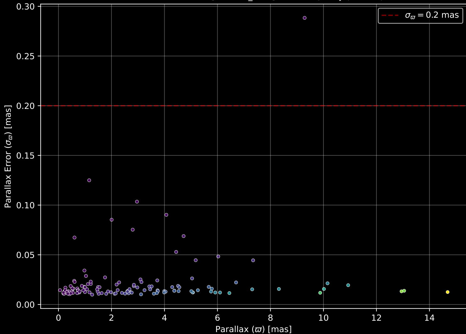
APOGEE DR17 Field: [042+45_MGA] Parallax Quality (n= 135)
